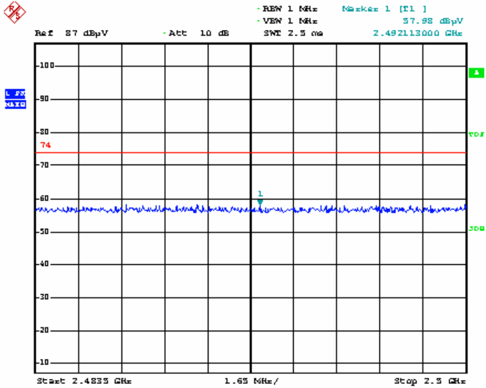
802.11b high channel Hor Peak
