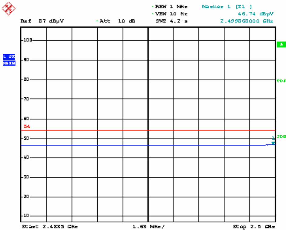
802.11g high channel Hor Peak
