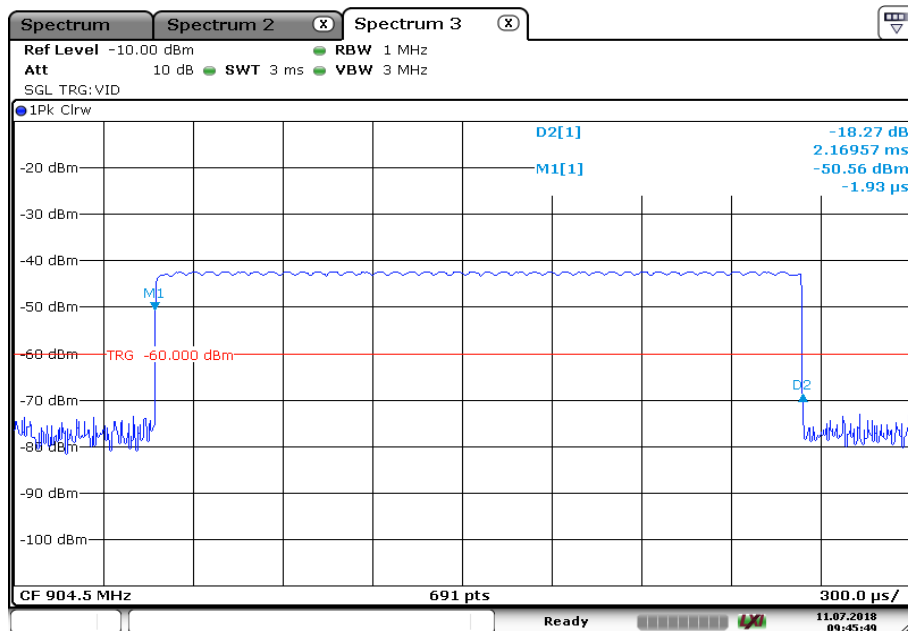
Plot 1: Time slot length = 2.17 ms
