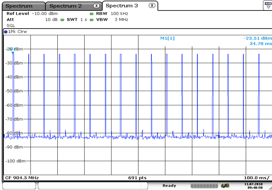
Plot 2: Number of hopping channels in 1s = 17
