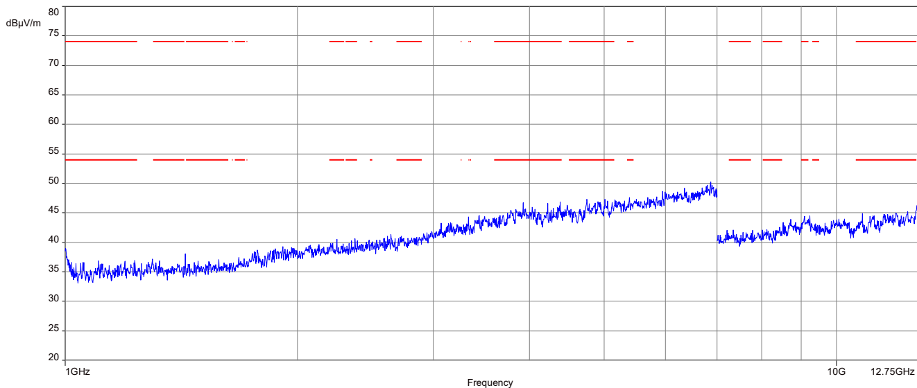
Plot 4: 1GHz – 12.75 GHz, RX-Mode, horizontal & vertical polarisation
