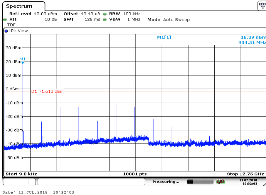
Plot 1: Low channel, 9 kHz – 12.75 GHz BSP!
