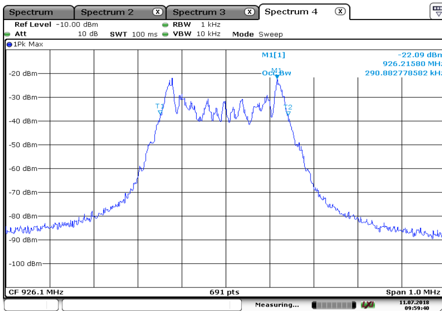
Plot 6: High channel; 99% bandwidth
