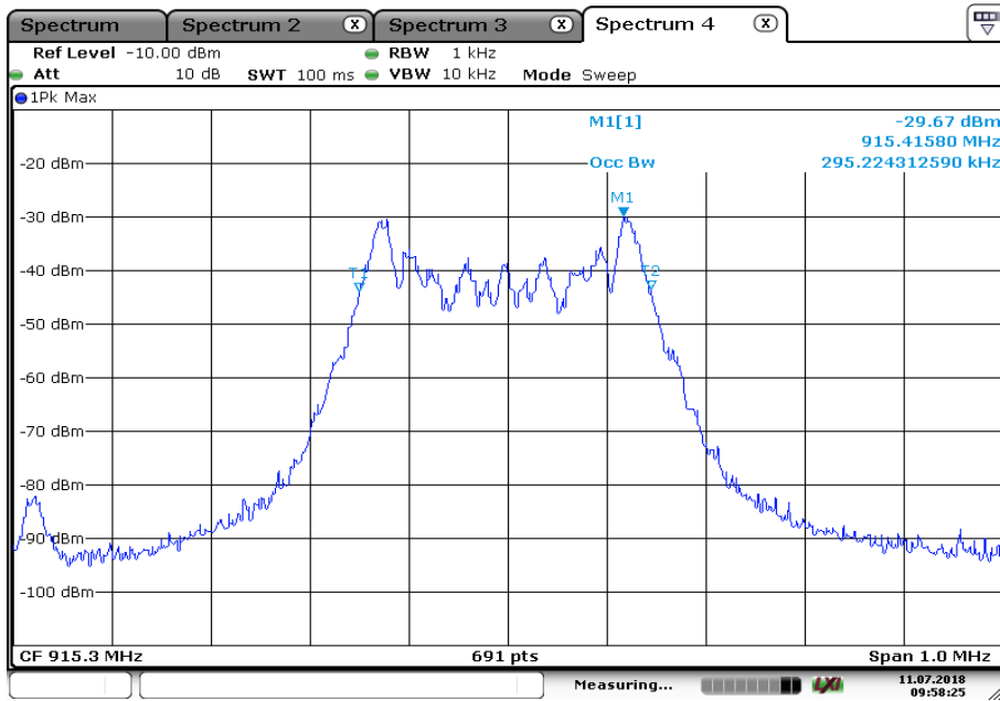
Plot 4: Middle channel; 99% bandwidth
