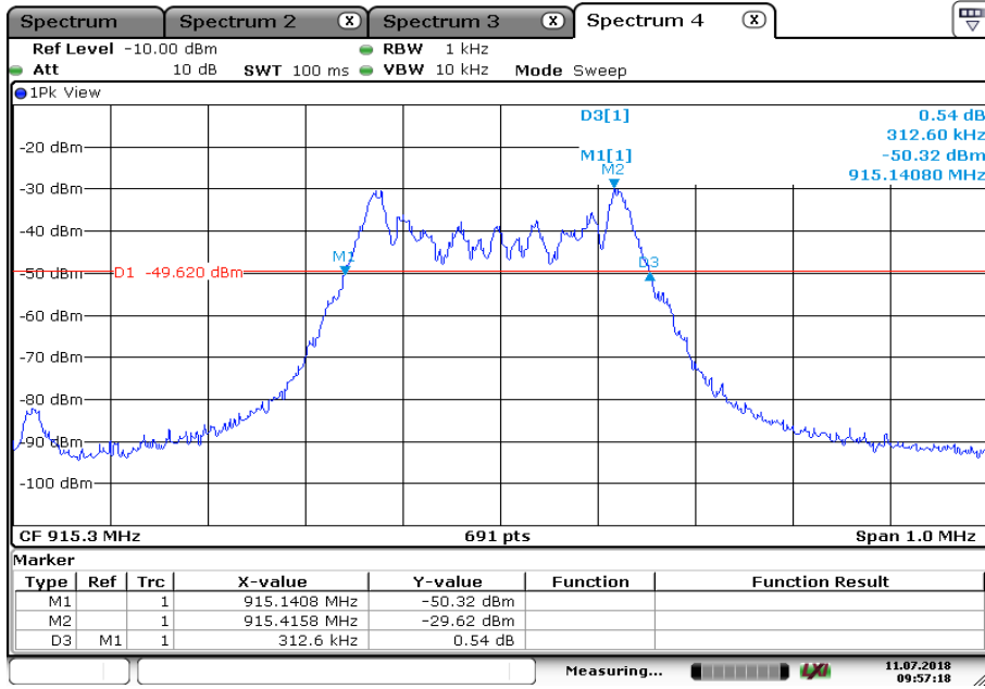
Plot 3: Middle channel; 20 dB-bandwidth
