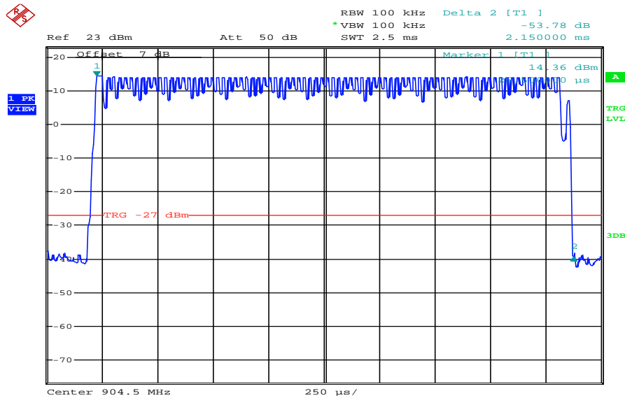
Plot 7: Time slot length = 2.15 ms
