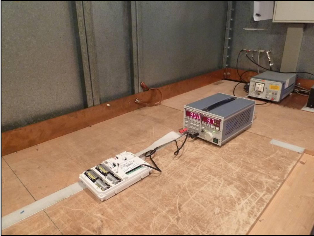
Photo 3: conducted emission
