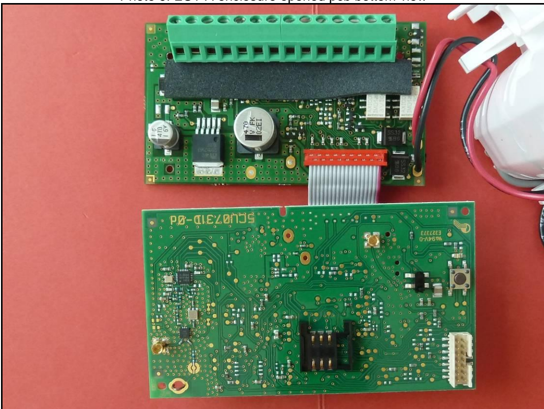
Photo 9: EUT A enclosure opened pcb bottom view
