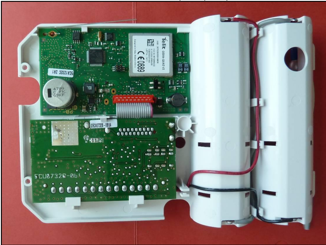
Photo 8: EUT A enclosure opened pcb top view
