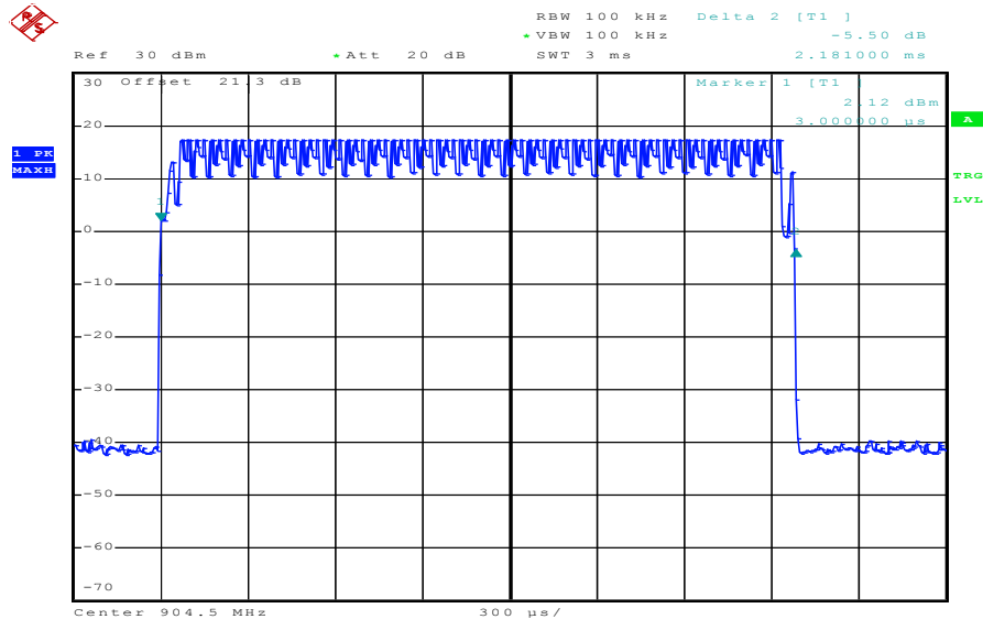
Plot 25: Time slot length = 2.181 ms
