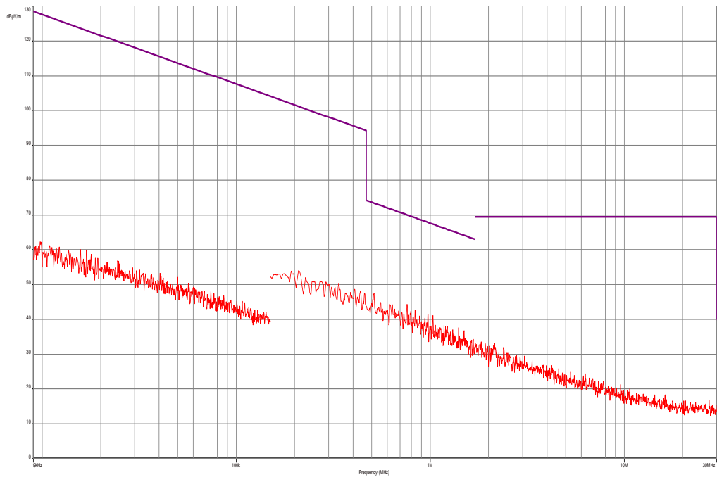
Plot 18: RX - mode
