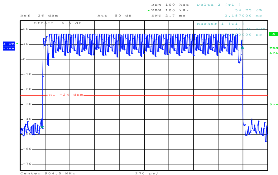
Plot 7: Time slot length = 2.187 ms
