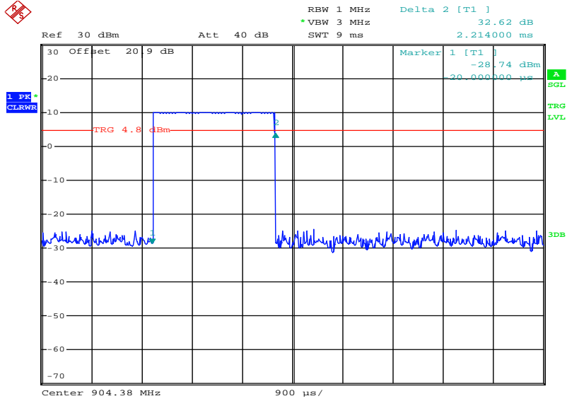
Plot 1: Time slot length = 2.214 ms
