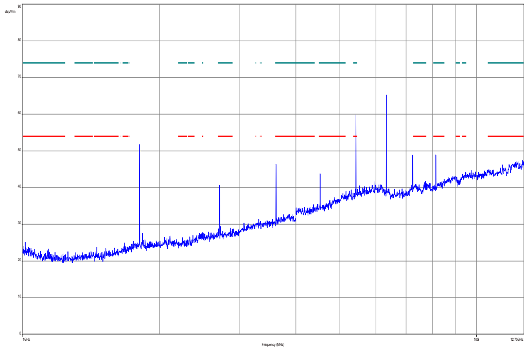
Plot 2: 1 – 12.75 GHz, horizontal & vertical polarisation (lowest channel)
