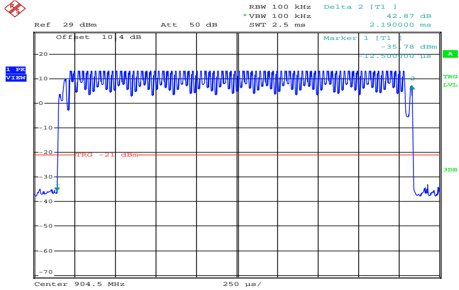
Plot 1: Time slot length = 2.19 ms
