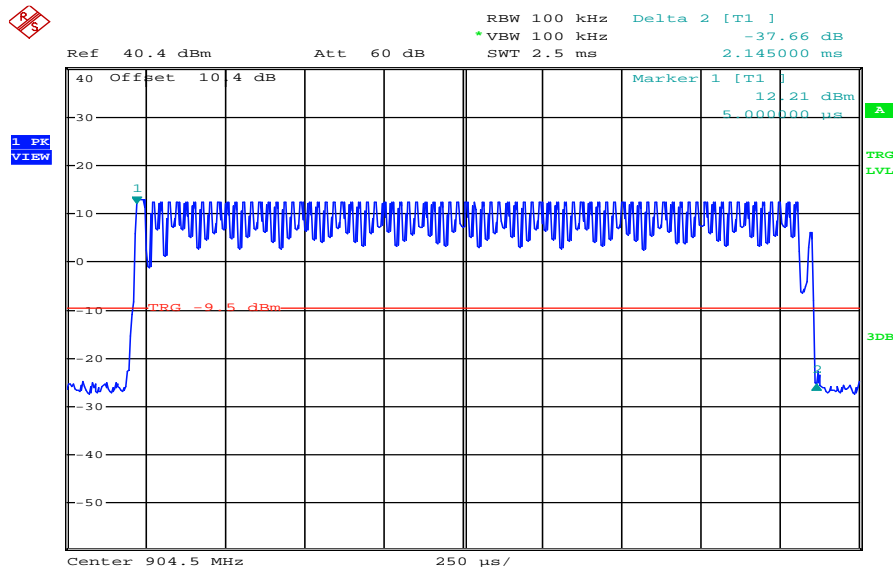
Plot 7: Time slot length = 2.145 ms
