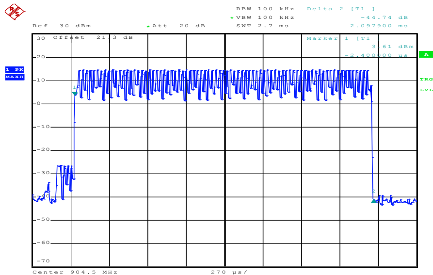
Plot 25: Time slot length = 2.0979 ms
