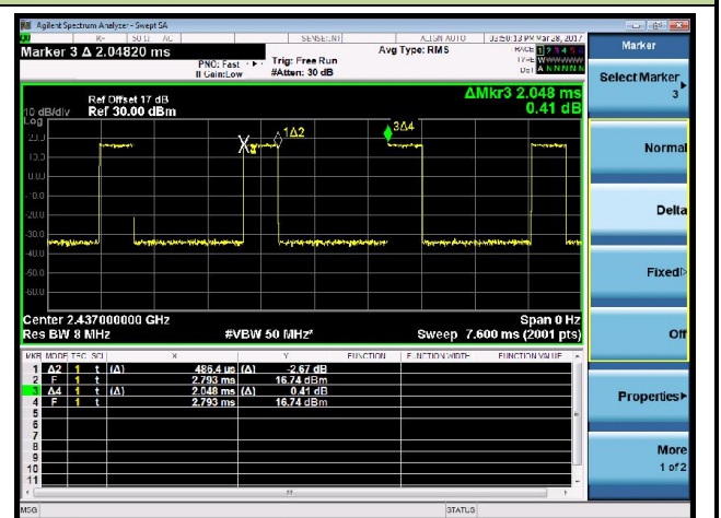
802.11g - Duty Cycle
