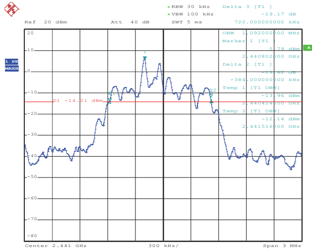
Figure 5: 20dB Bandwidth, Mode B (2441MHz 8DPSK and GFSK)
