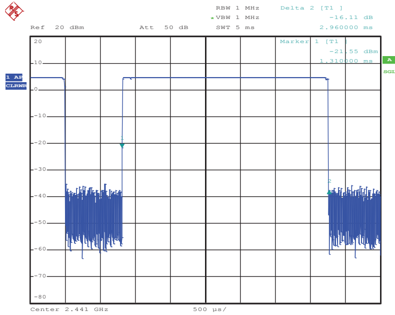
Figure 13: Dwell Time, Mode G(Hopping), 2M-DH5, Mid channel
