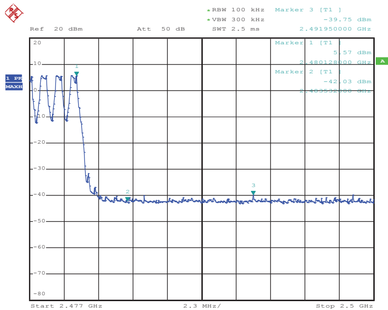
Figure 24: Upper Band Edge Conducted, Hopping Enabled
