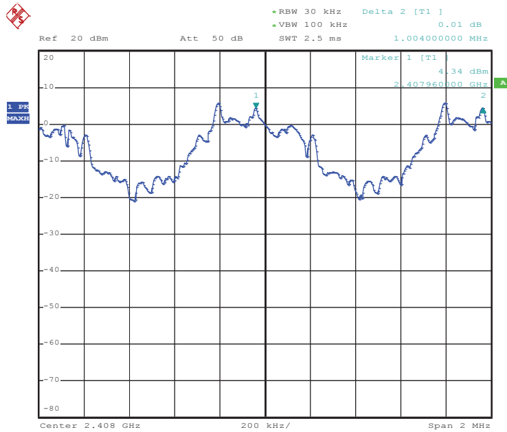
Figure 1: Carrier Frequency Separation-Low Channel
