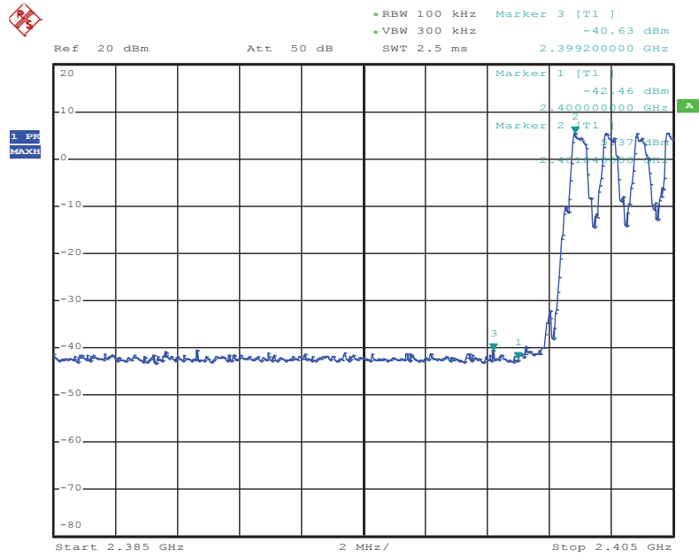
Figure 23: Lower Band Edge Conducted, Hopping Enabled
