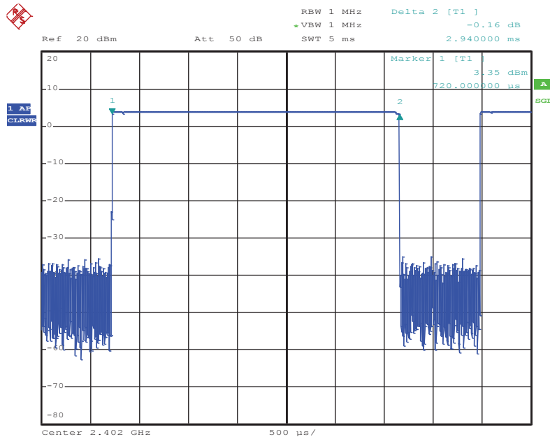
Figure 12: Dwell Time, Mode G (Hopping), 2M-DH5, Low channel
