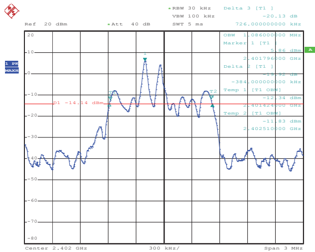
Figure 7: 99% Bandwidth, Mode A (2402MHz 8DPSK and GFSK)
