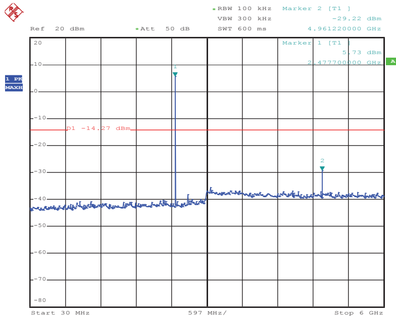
Figure 19: Conducted Spurious Emission, 30MHz – 6GHz, Mode C (2480MHz)
