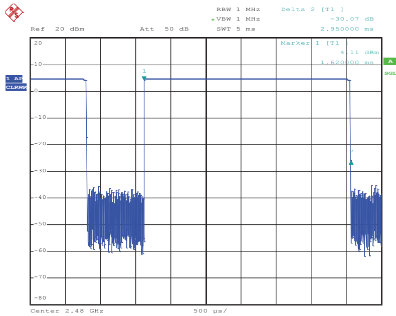
Figure 14: Dwell Time, Mode G(Hopping), 2M-DH5, High channel
