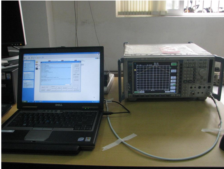
Photograph 4: Set-up for Conduct Power
