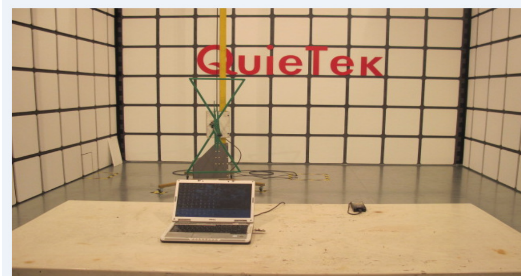
Photograph 2: Set-up for Radiated Emission, 30MHz-1000MHz
