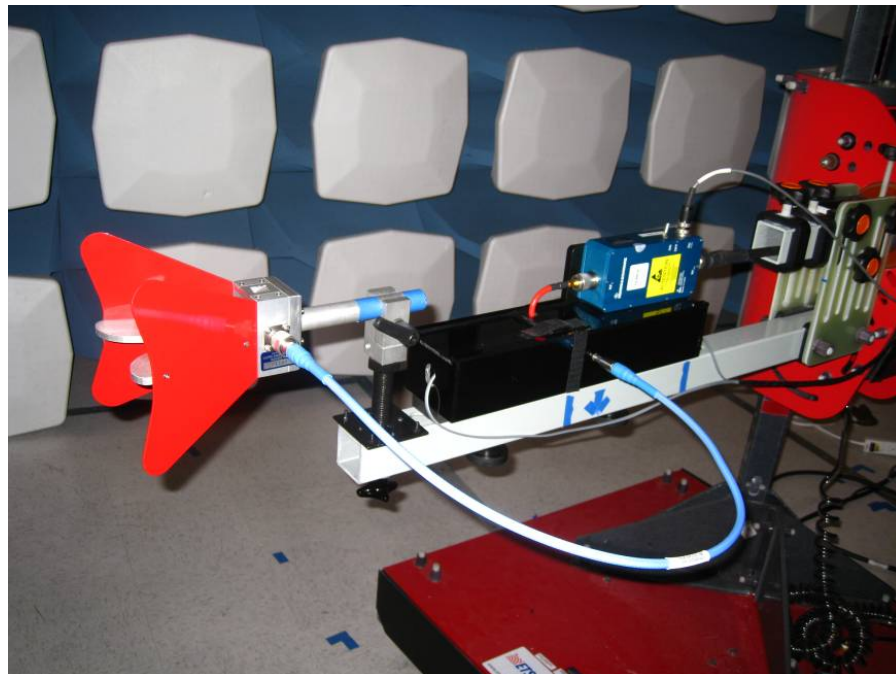
PHOTOGRAPH SHOWING THE EUT CONFIGURATION FOR RADIATED EMISSIONS
