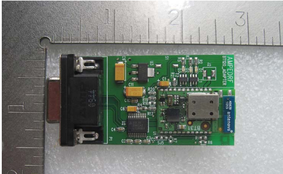
Top view of EUT on supported PCB
