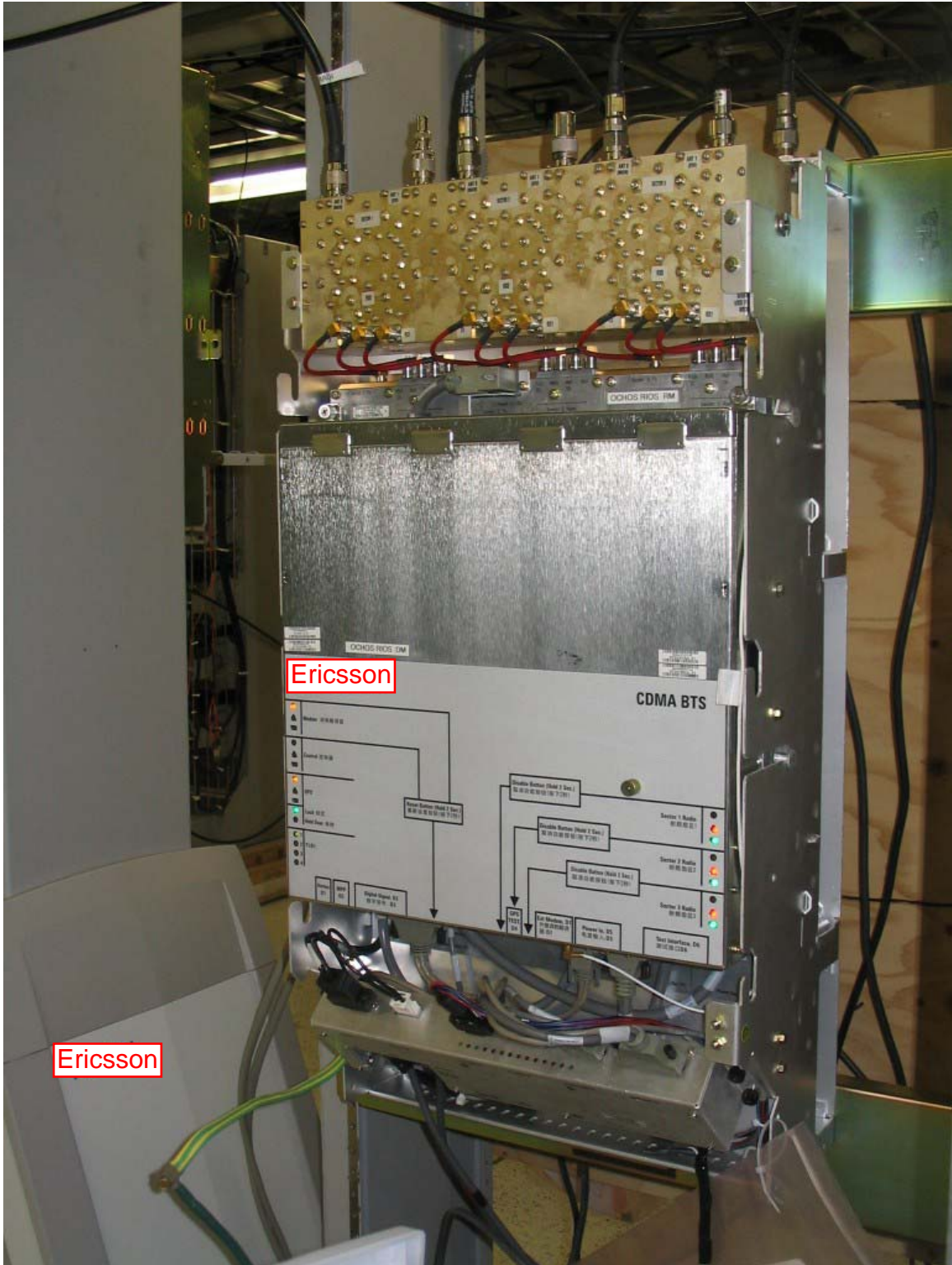
Right Front Side View With Cover OFF
