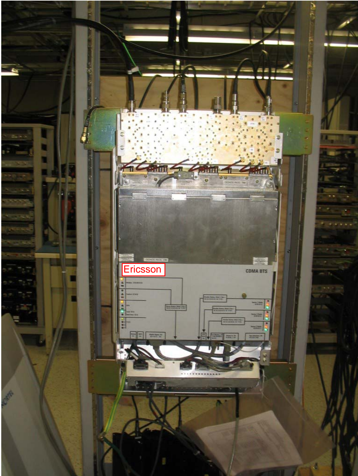
Front View With Cover OFF
