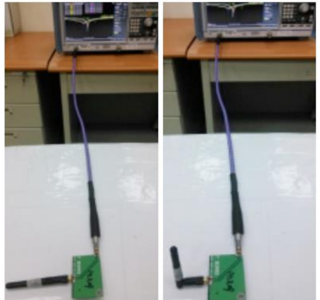
Antenna straight
