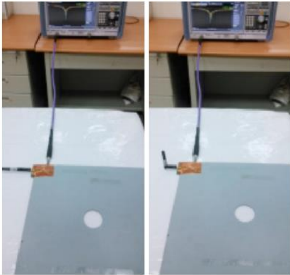
Antenna straight
