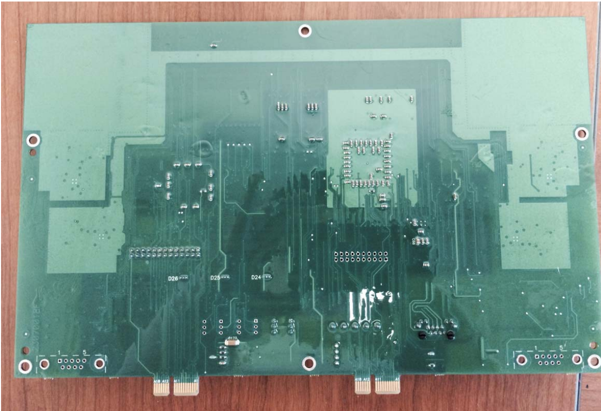
Bottom Side PCBA
