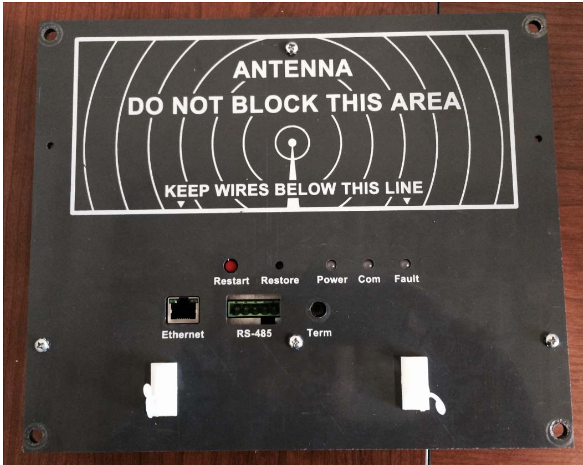
PCB installed onto PVC Panel
