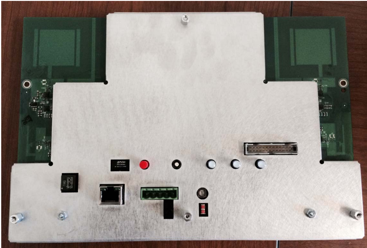
Top Side PCBA with Shield Installed
