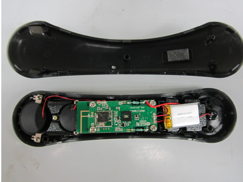
1.1.5 Front view 1
