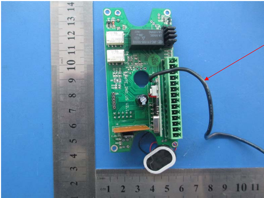
EUT (Receiver)-PCB 1 Rear View
