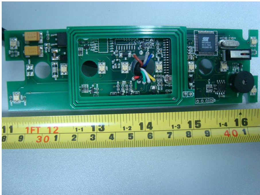
EUT – Main Board with Antenna Top View
