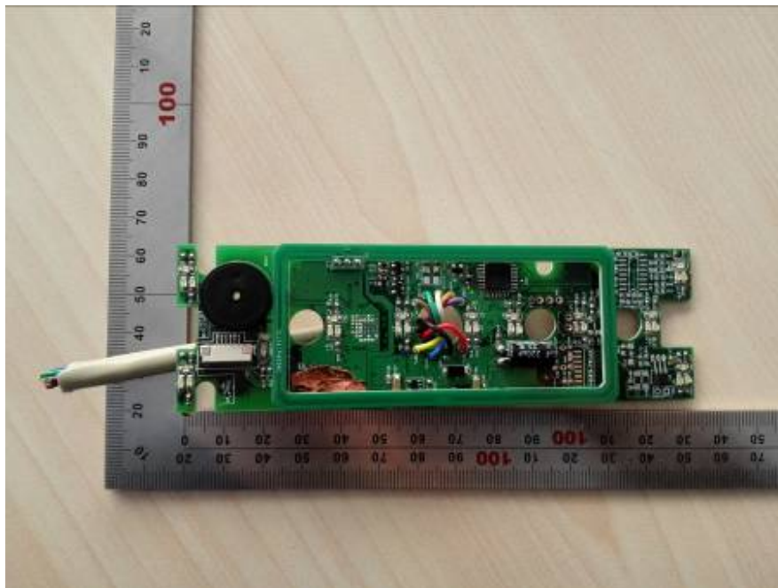
EUT – Main Board Top & Loop Antenna View
