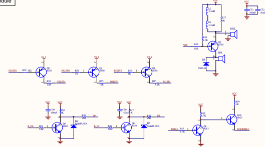
Driver Module
