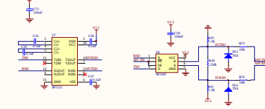
Communication Module
