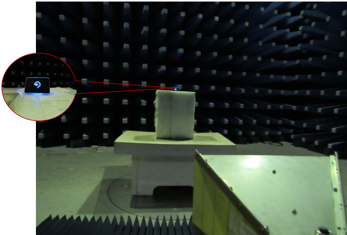
Radiated Emissions Setup Above 1GHz Front View
