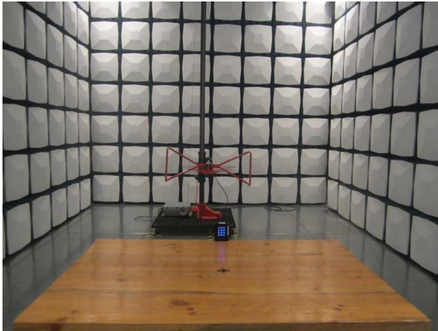
Radiated Emission 30 - 1000 MHz – Front View
