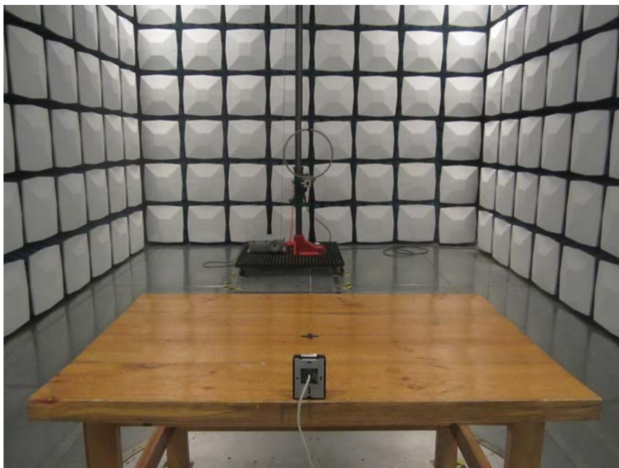
Radiated Emission 9 kHz - 30 MHz – Rear View
