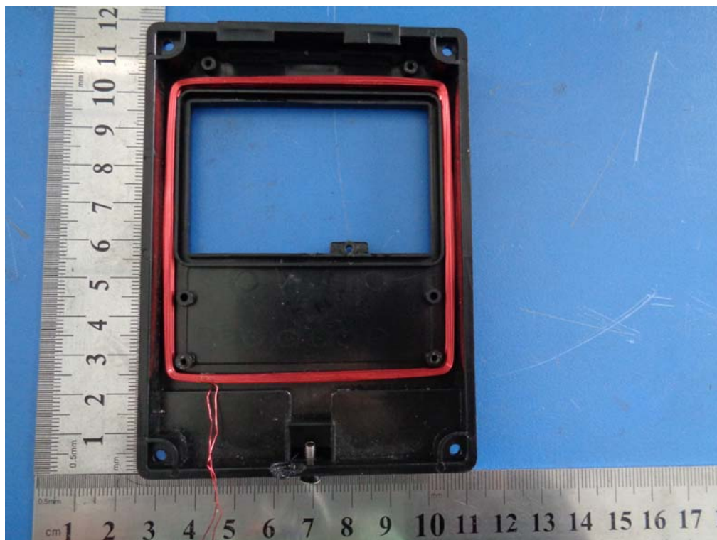
Antenna – Front View(125kHz)
