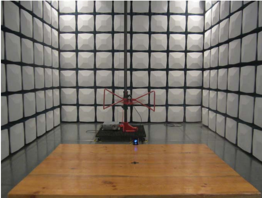
Radiated Emission (30 MHz-1 GHz)- Rear View
