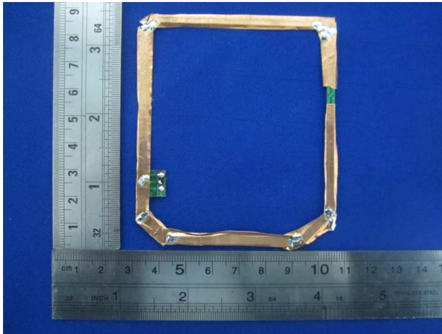
EUT -13.56MHz Antenna Top View
