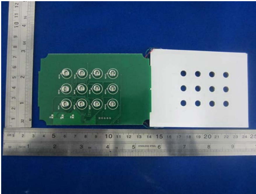
EUT –Touch Board Uncover View
