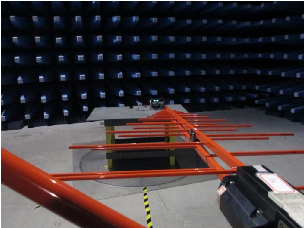
Radiated Spurious Emissions Test Setup (30MHz - 1GHz) - Front View
