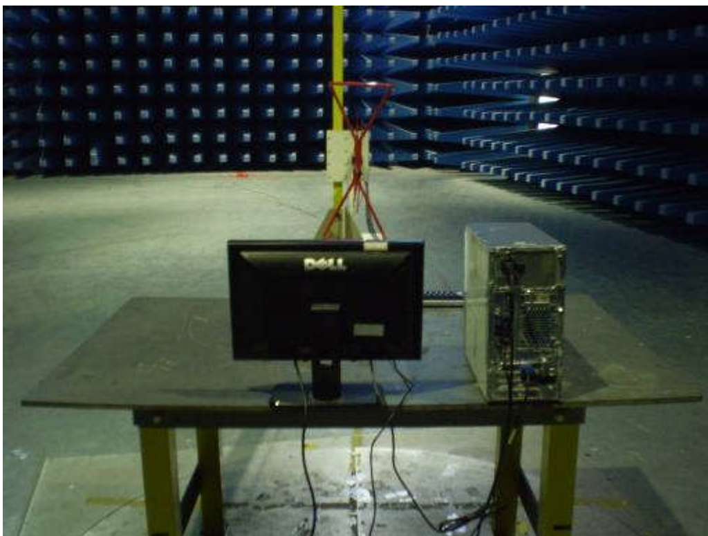
Radiated Emission Setup Rear View
