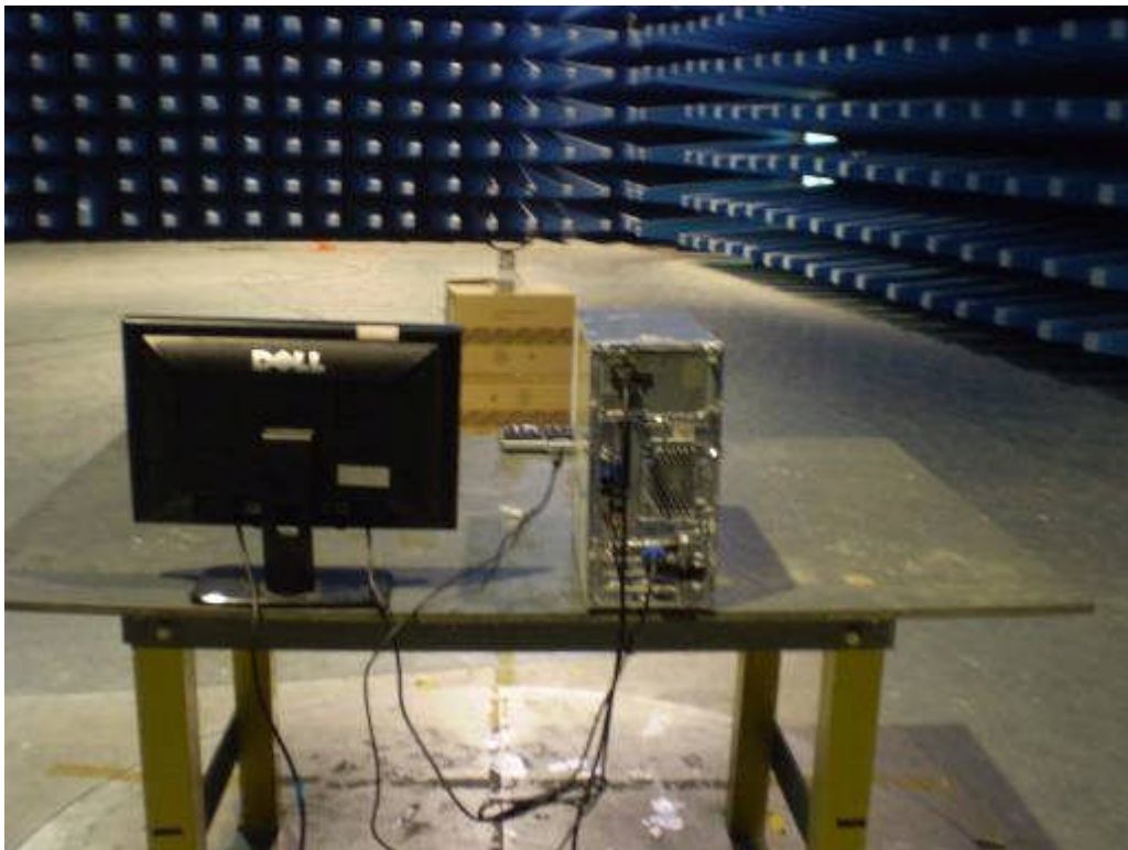
Fundamental Frequency Setup Rear View
