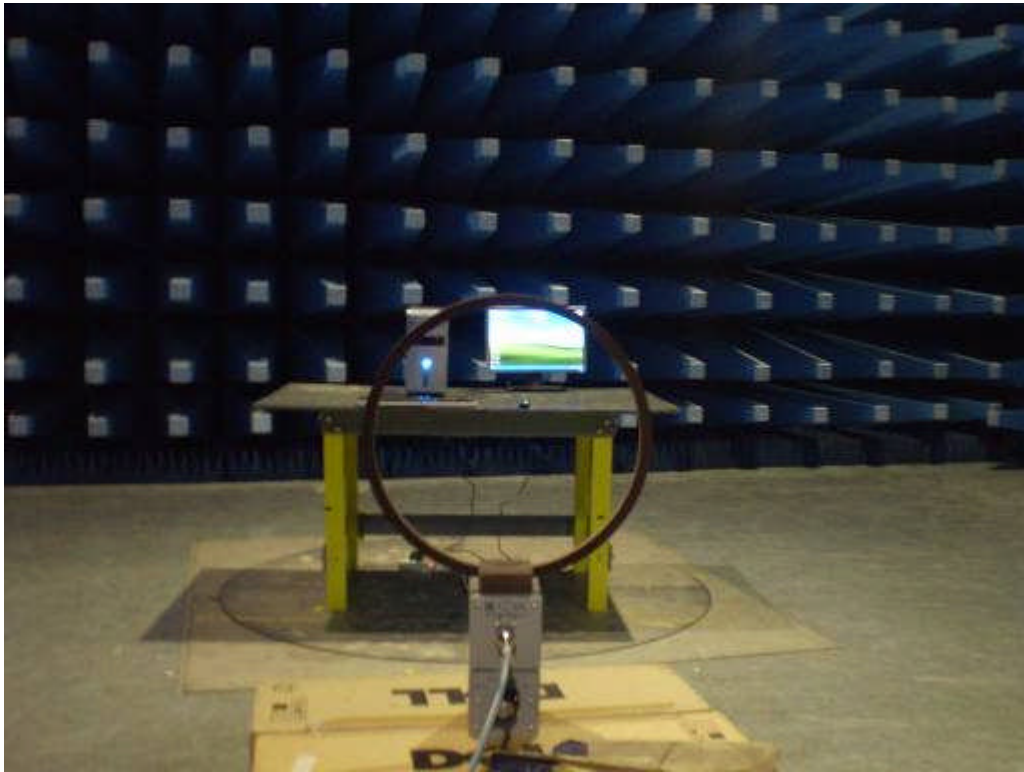
Fundamental Frequency Setup Front View
