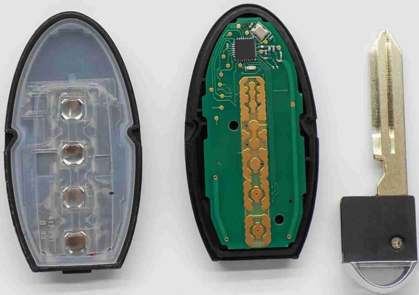
4 Button Assembly
