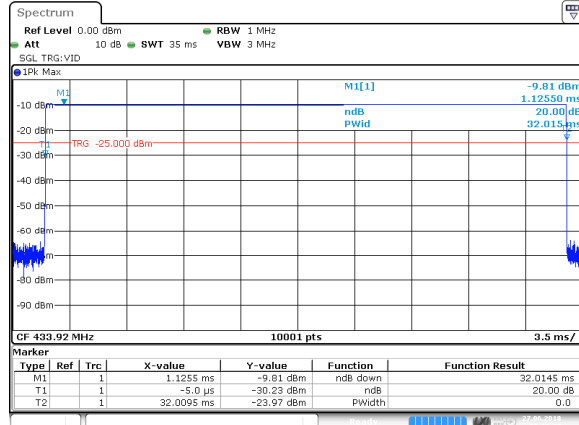
Figure 7.5.2-2: Duty Cycle (Pulse Width)
