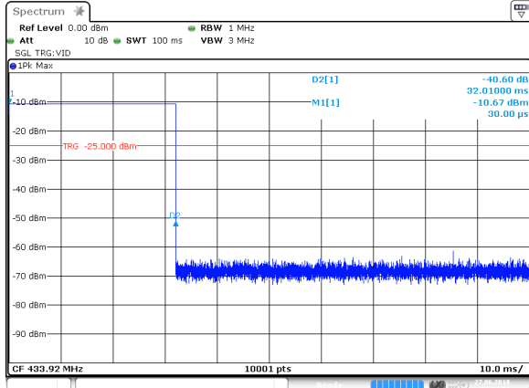
Figure 7.5.2-1: Duty Cycle (100ms)
