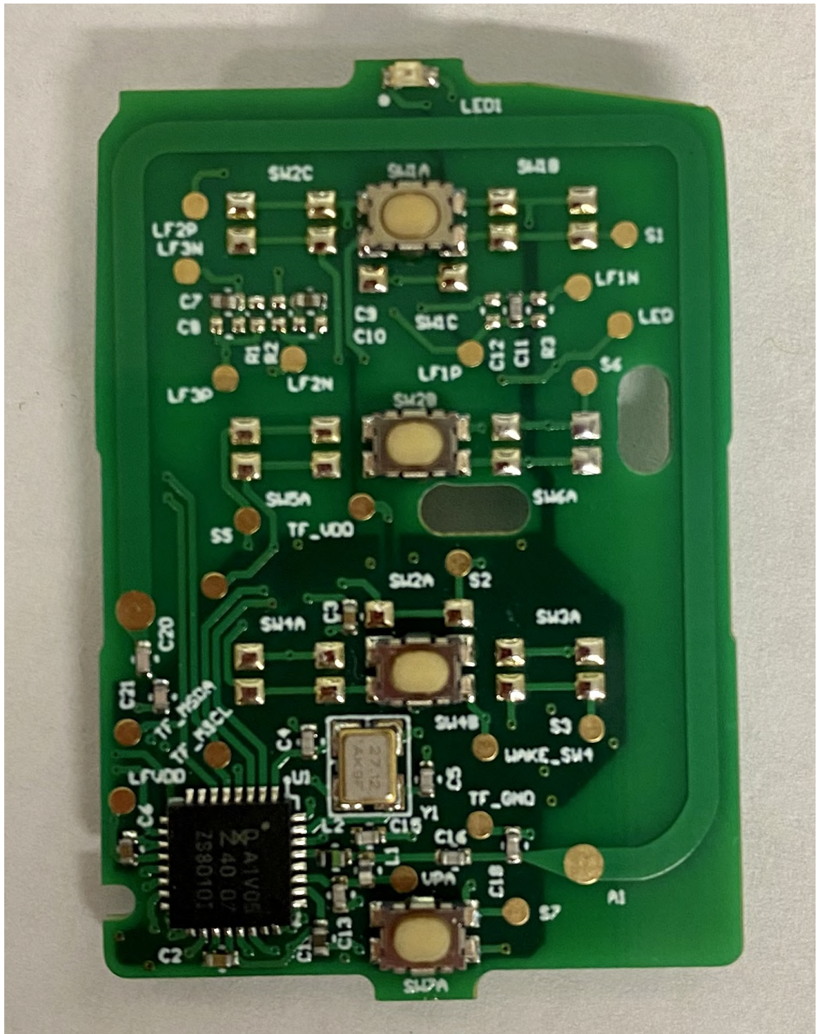
Assembly parts
