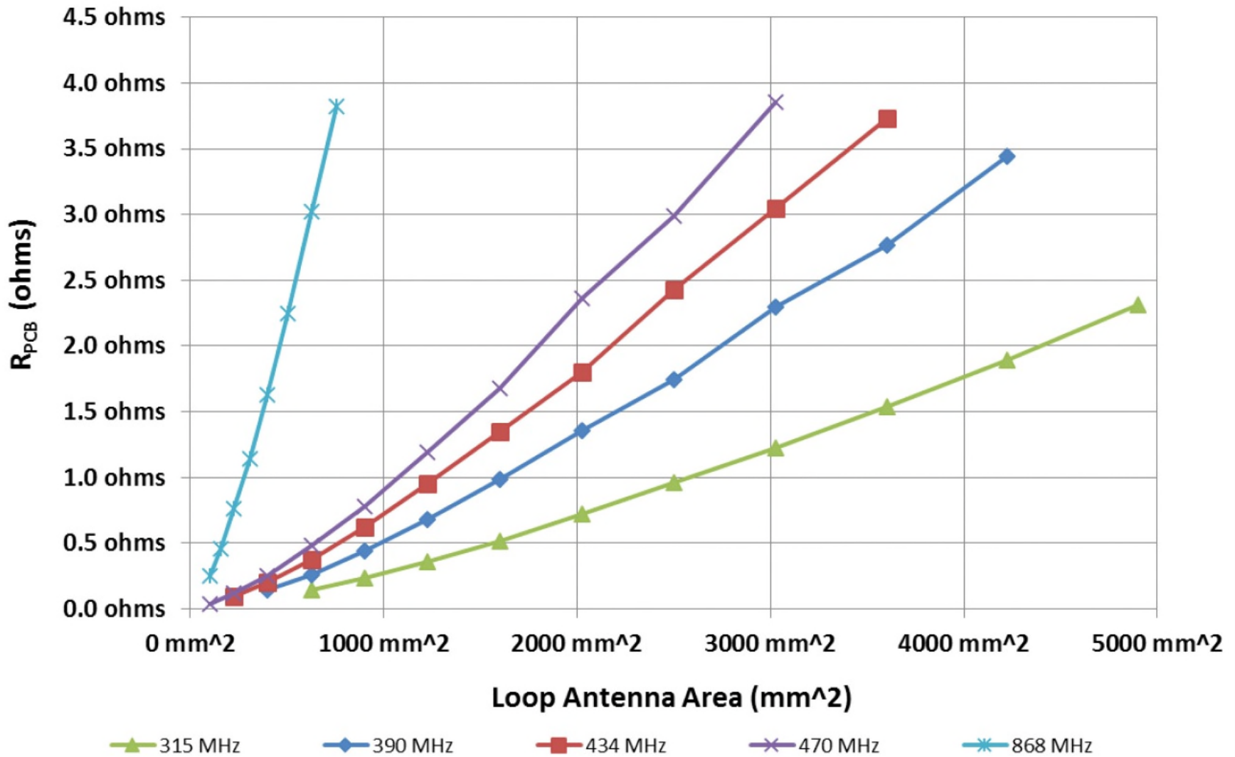
Figure 2. Dielectric Loss Resistance R PCB vs. Area vs. Frequency
