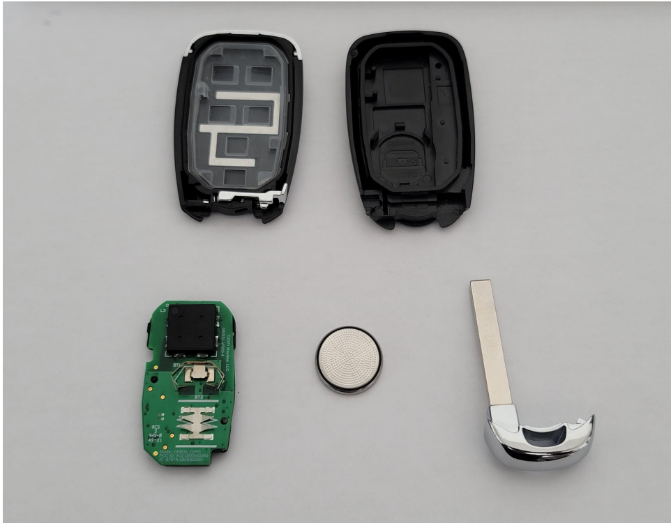
GMSSL-G060 Internal Photos - BOTTOM
