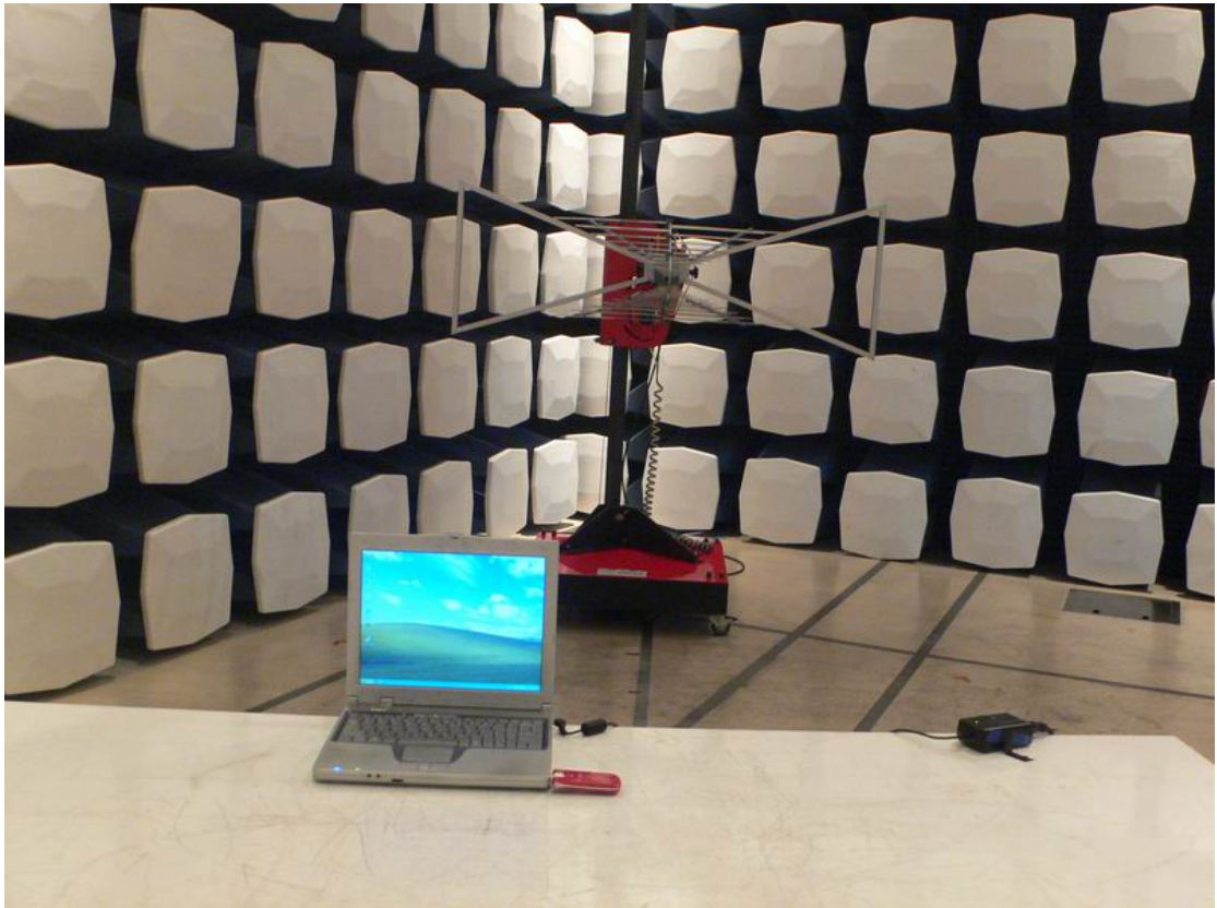
Radiation Test Setup
