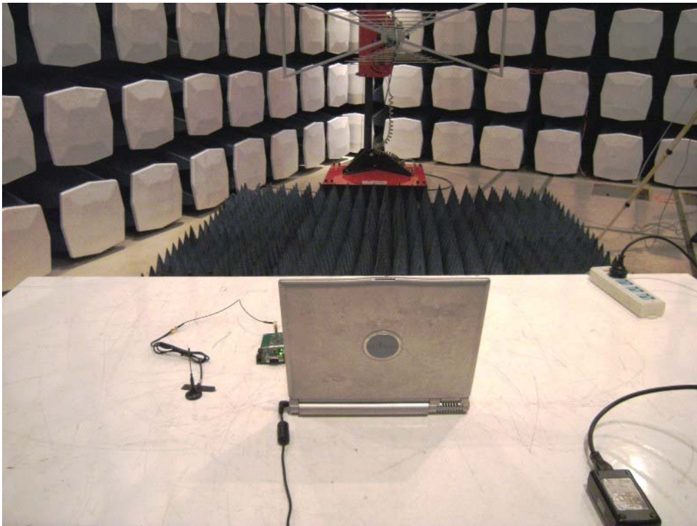
Radiation Test Setup 1
