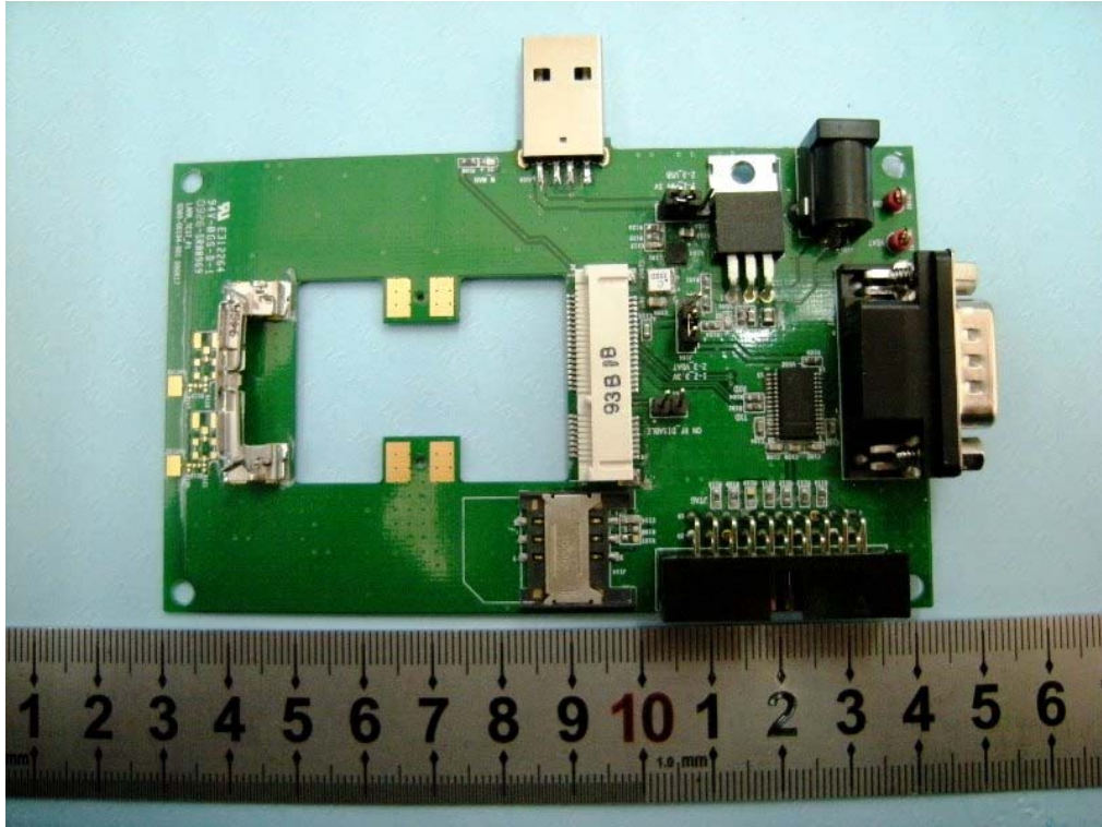
TEST BOARD FRONT
