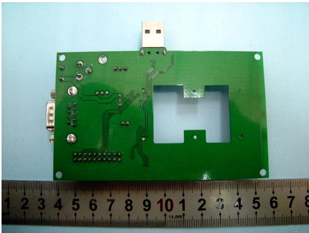
TEST BOARD BACK
