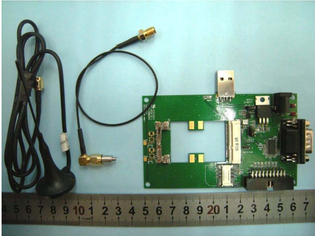
TEST BOARD+ANTENNA+RF CABLE
