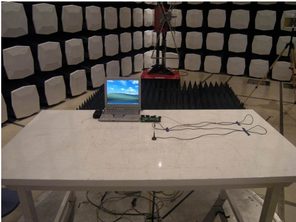
Radiation Test Setup
