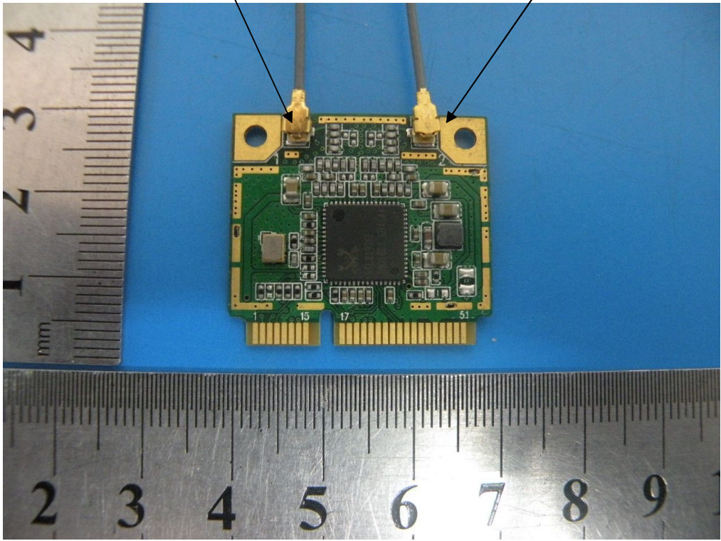
Port 1 WIFI Antenna
