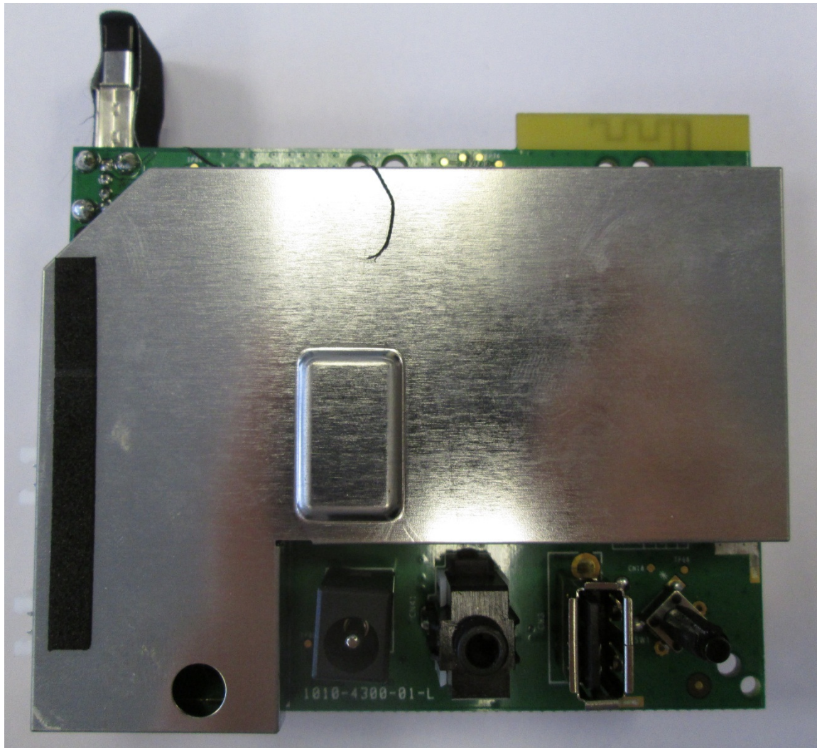
Main PCB Rear (with screening can)
