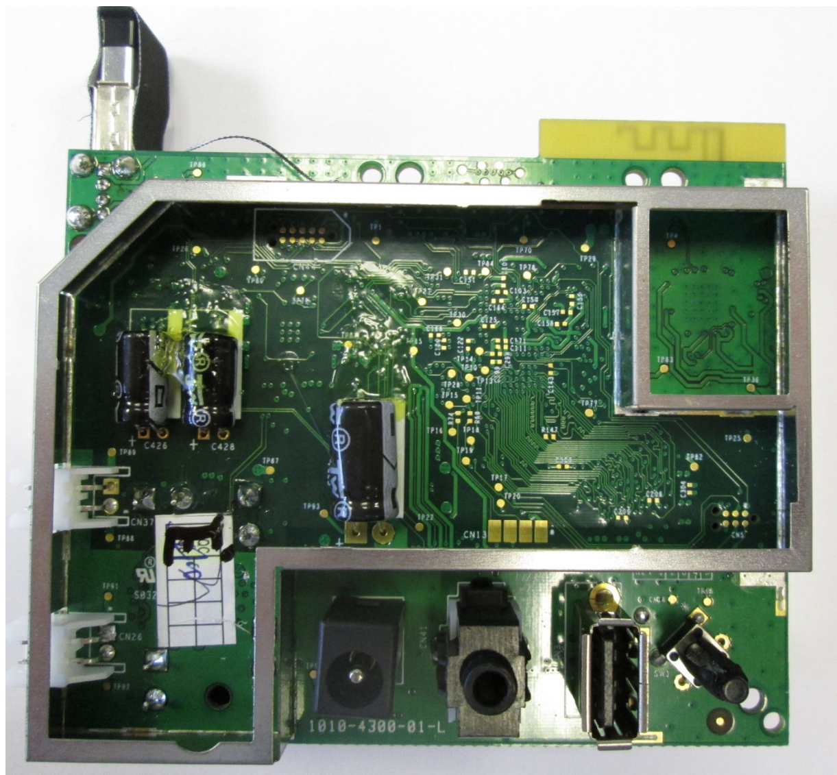
Main Screening Can Rear (without screening can)
