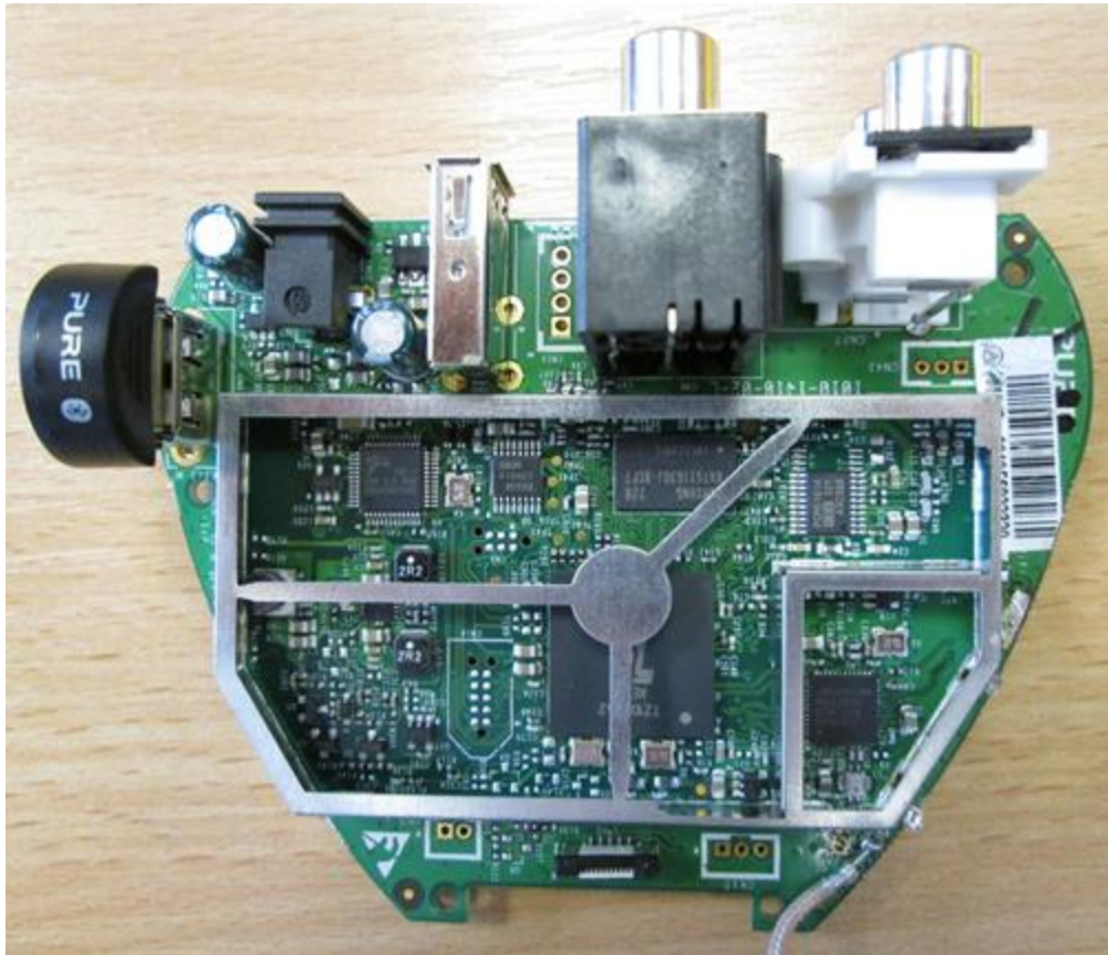
Main PCB top (without screening can)
