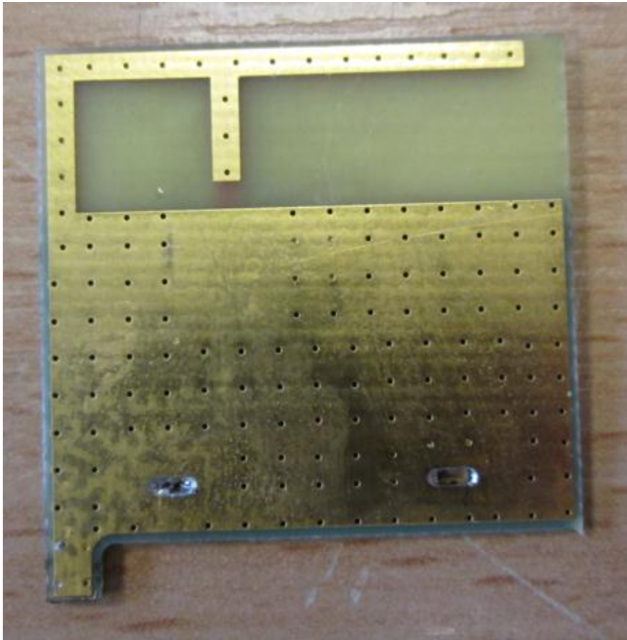
WiFi antenna PCB Rear
