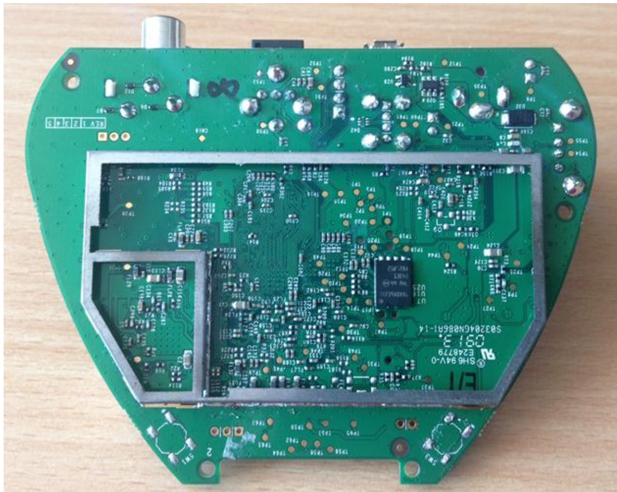
Main PCB bottom (without screening can)
