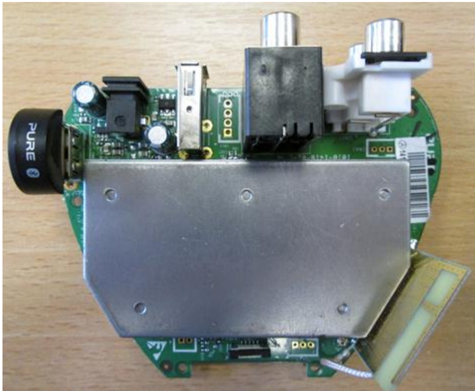
Main PCB top (with screening can)
