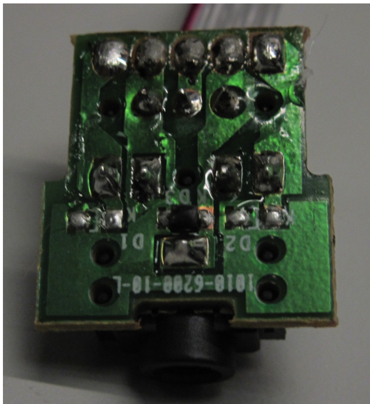
Auxiliary in PCB Bottom
