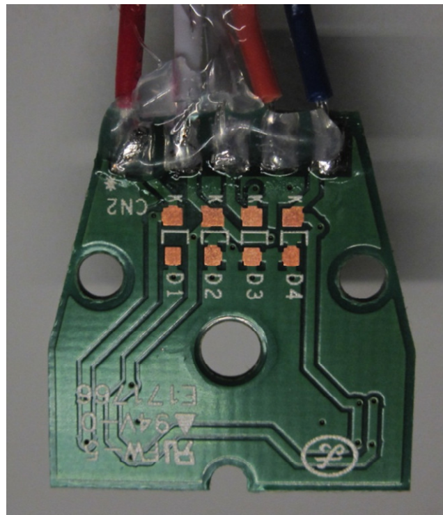
Volume Buttons PCB Bottom
