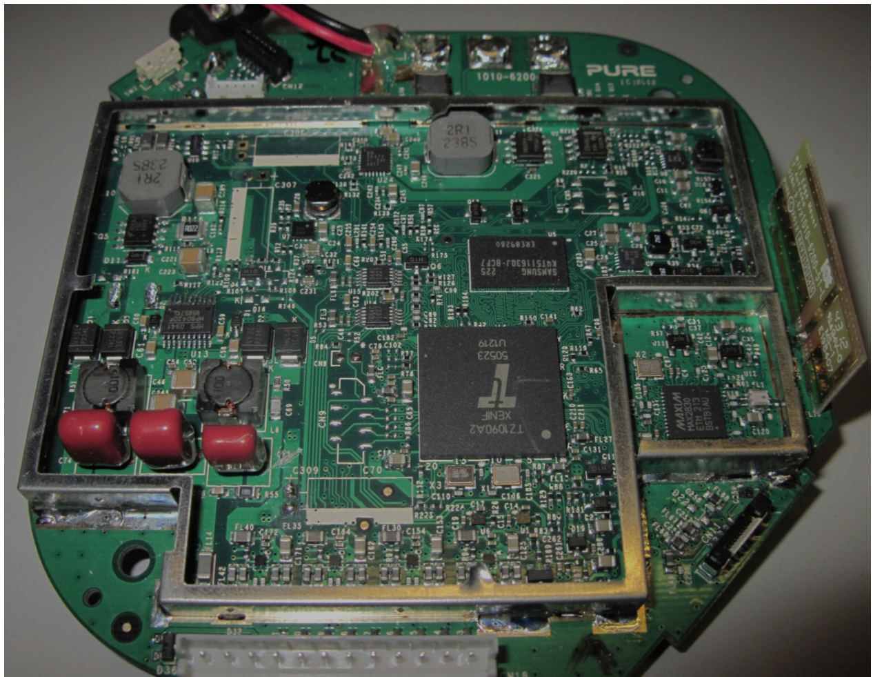
Main PCB top (without screening can)
