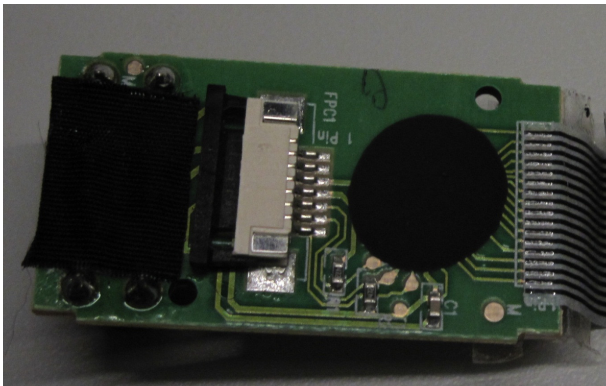
LCD PCB Bottom
