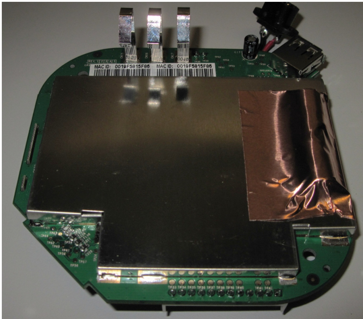
Main PCB bottom (with screening can)
