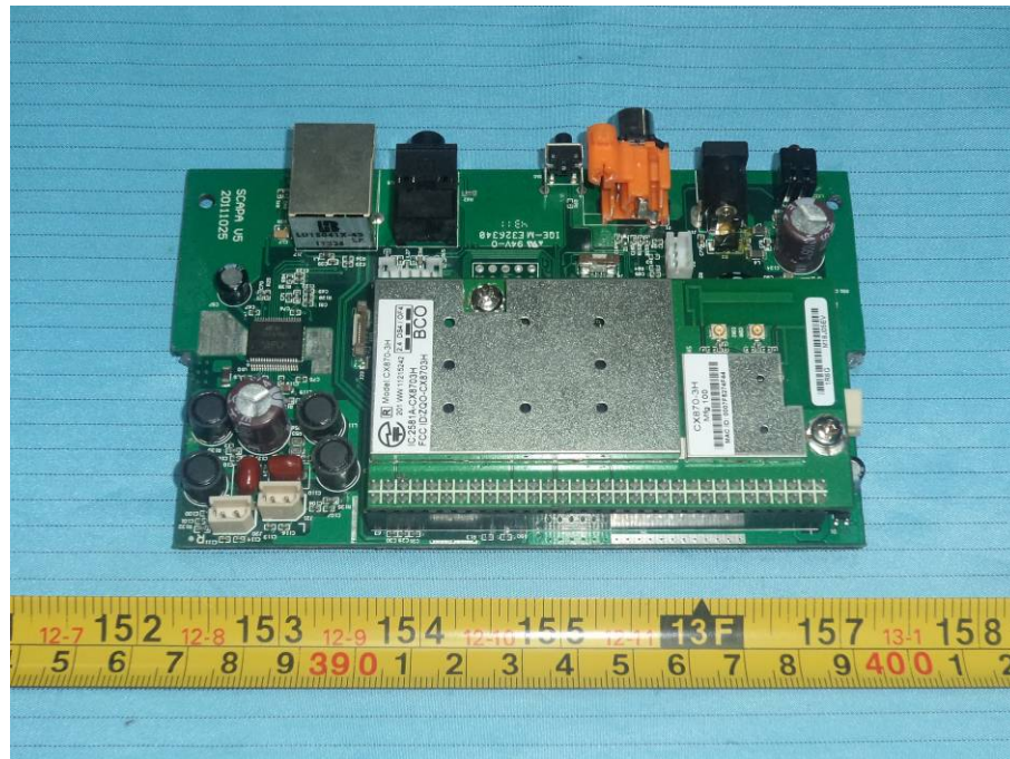
EUT – Main Board with RF Module View
