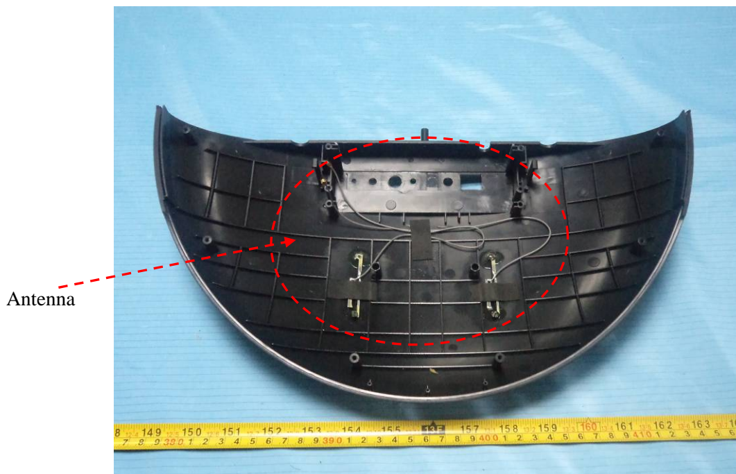
EUT –RF Antenna View
