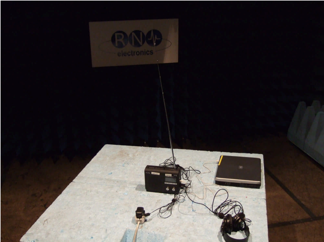
Radiated emissions 2
