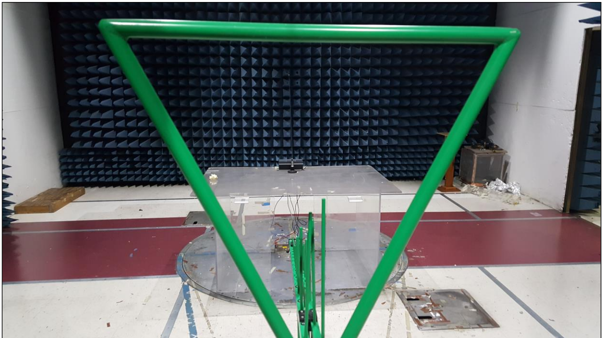
Photograph 2. Field Strength of Spurious Emissions, Setup 30 MHz - 1 GHz
