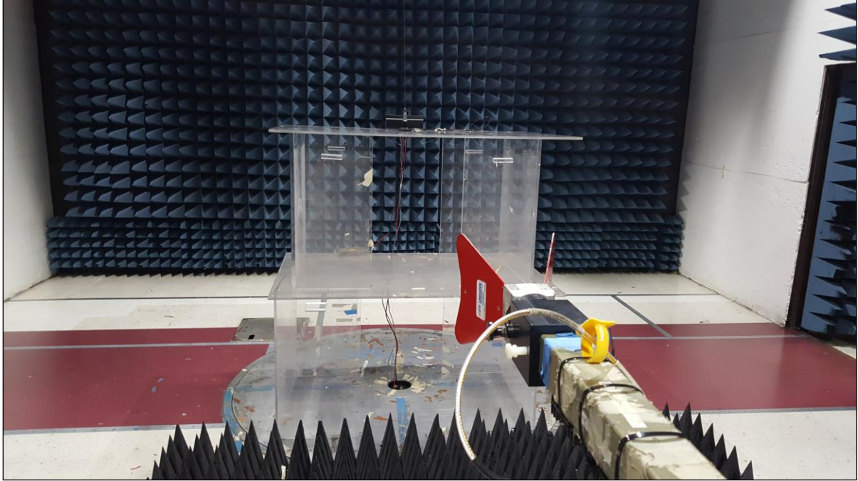
Photograph 1. Field Strength of Spurious Emissions, Setup Above 1 GHz
