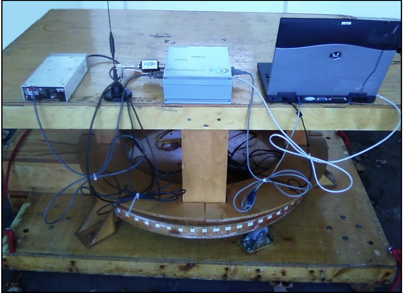
Photograph 2: Radiated Testing – Back View
