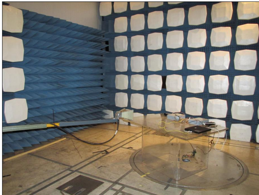
Photograph 2. Radiated Emissions, Test Setup, Above 1 GHz
