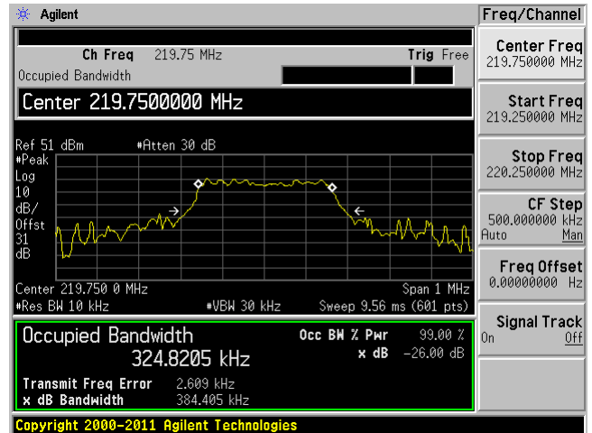
Channel 4, 219.75MHz
